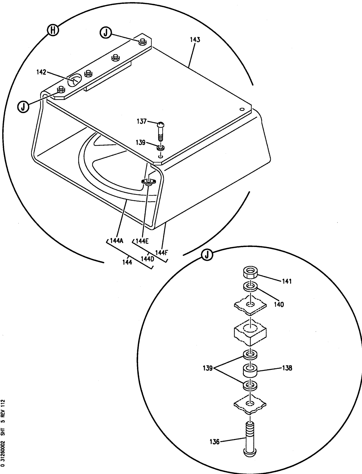
MODULE ASSY-AURAL WARNING 31-26-00 FIGURE: 02 SHEET: 005
