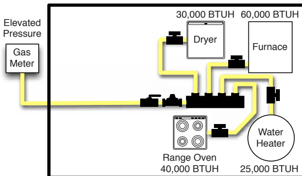
Figure 3.4 A dual pressure system layout
