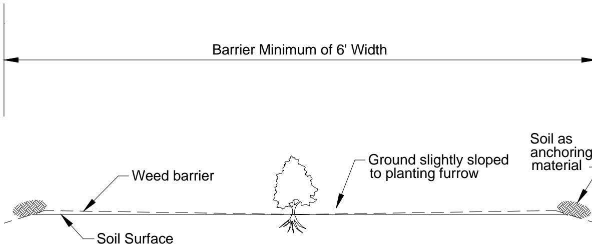
Side View
