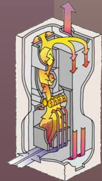
The combustion system at a glance. (Exploded view)
