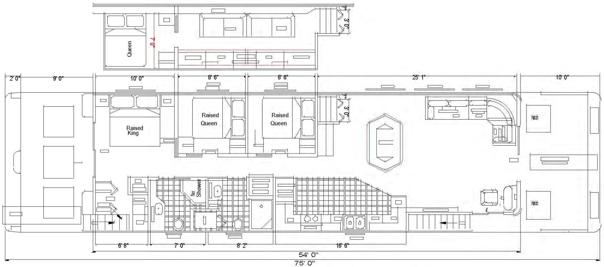
Canyon Cabana — Main Deck 18' x 75'
