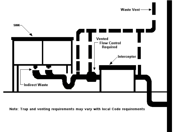
Figure A1.5.13- Interceptor Serving Sink with Indirect waste
