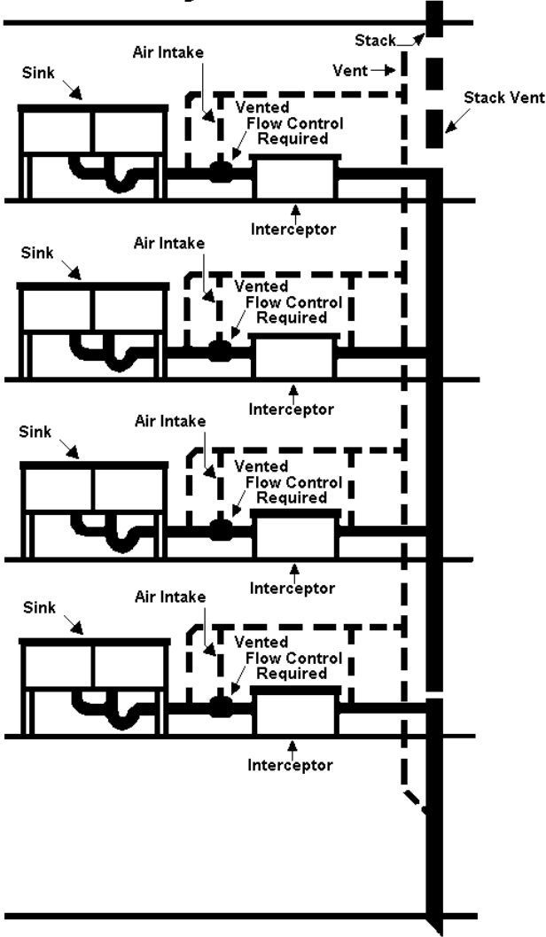
Figure A1.5.5- Interceptors Serving Trapped & Vented Sinks-Flow Control Air Intakes Intersect Vent
