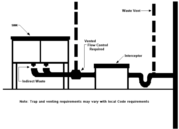
Figure A1.5.14- Interceptor Serving Sink with Indirect waste
