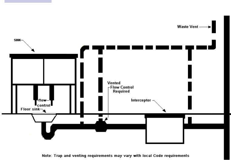
Figure A1.5.11- Interceptor Serving Sink with Indirect waste
