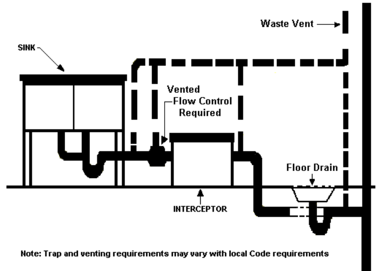
Figure A1.5.10- Interceptor Serving Sink protected from waste with Floor drain
