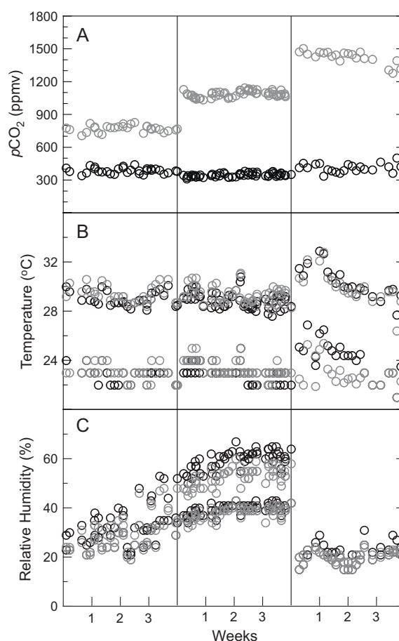
Fig. 1. p\text{CO}_2 (A), temperature (B), and relative humidity (C) conditions for three ambient (black) and three elevated (gray) p\text{CO}_2 experiments. Within the growth chambers, p\text{CO}_2 and temperature conditions were controlled; relative humidity fluctuated naturally. The mean and standard deviation for all experiments are presented in Table S1.
