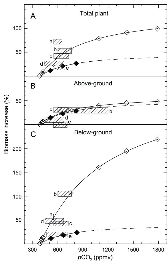
Fig. 2. Percent-biomass-increase observed for R. sativus across the full range of atmospheric p\text{CO}_2 levels estimated for the next 300 years (348–1791 ppmv) compared with previous results on root crops (a, Daucus carota , carrot; b, Raphanus sativus , radish; c, Beta vulgaris , sugar beet; d, Ipomoea batatas , sweet potato; e, Solanum tuberosum , potato) and herbaceous species (Hunt et al., 1991, 1993) at lower p\text{CO}_2 levels. Percent-biomass-increase curves for this study (open diamonds) were calculated from the fitted hyperbolic functions for biomass (Eqs. (1) and (2) within text) using an ambient p\text{CO}_2 level of 389 ppmv (present p\text{CO}_2 level). Percent-biomass-increase curves (closed diamonds) were calculated using Eq. (1) and the mean a and b values reported for 23 responsive ( b < 1 , total biomass) herbaceous species (Hunt et al., 1991, 1993). Open diamonds (this study) and closed diamonds (Hunt et al., 1991, 1993) mark p\text{CO}_2 levels under which the plants were grown; dashed lines extrapolate data from Hunt et al. (1991, 1993). Root crop data (shaded bars) were compiled from published data on dry biomass following the methods of Poorter (1993). Data were restricted as follows: (1) only data from the vegetative phase were used, (2) only experiments with control p\text{CO}_2 -levels between 300 and 450 ppmv and elevated p\text{CO}_2 -levels less than 2000 ppmv were used, in order to make a direct, quantitative comparison with data from this study, (3) for studies in which multiple environmental variables were tested (i.e., ozone, water availability, irradiance, etc.), biomass data were collected from experiments in which control plants grew best, and (4) for studies with multiple harvest dates, only data from the final harvest were used. These criteria resulted in a total of 127 observations of percent biomass increase ( n = 38 , above ground; n = 45 , below ground; n = 44 , total biomass) (see Table S2). Data for root crops extend the range of elevated p\text{CO}_2 levels tested and mark the average biomass increase, relative to ambient p\text{CO}_2 levels. (A) Total biomass (sugar beet, n = 14 ; carrot, n = 3 ; sweet potato, n = 5 ; radish, n = 10 ; potato, n = 12 ). Except for potato (e), total percent biomass increases greater for root crops (shaded bars) than non-crop species (closed diamonds). Note that the average, percent-total-biomass-increase at lower p\text{CO}_2 levels for Raphanus from previous studies (shaded bar, b) is similar to that observed in this study (open diamonds), but the percent increase in total biomass at very high p\text{CO}_2 levels observed in this study exceeds the extrapolated data of Hunt et al. (1991, 1993) (dashed curve). (B) The above-ground response for root crops (sugar beet, n = 10 ; sweet potato, n = 8 ; radish, n = 6 ; potato, n = 14 ) does not exceed the response of non-root species at any p\text{CO}_2 level. (C) Below-ground biomass fertilization for root crops (sugar beet, n = 10 ; carrot, n = 2 ; sweet potato, n = 5 ; radish, n = 6 ; potato, n = 22 ) at low p\text{CO}_2 levels (<800 ppmv) (except potato) greatly exceeds the average response of non-crops across the full range of p\text{CO}_2 levels; however, the difference between root and
