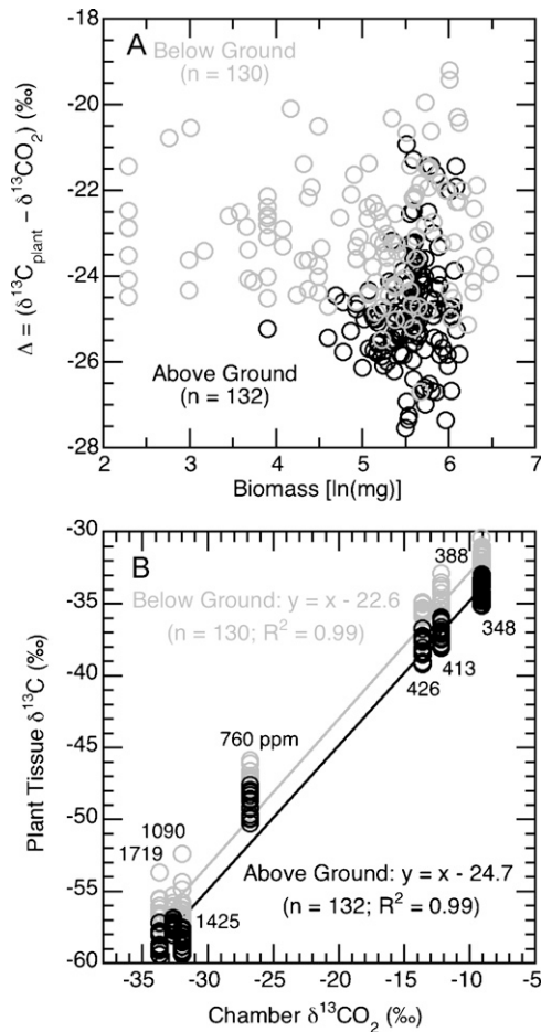
Fig. 3. Carbon isotope composition of plant tissue compared to plant biomass and to the carbon isotope composition of chamber \text{CO}_2 . Lack of correlation between (A) the net carbon isotope fractionation ( \Delta = \delta^{13}\text{C}_{\text{plant}} - \delta^{13}\text{CO}_2 ) and the amount of biomass produced contrasted with the strong correlation between (B) the carbon isotope composition of the plant tissue ( \delta^{13}\text{C}_{\text{plant}} ) and the carbon isotope composition of chamber \text{CO}_2 ( \delta^{13}\text{CO}_2 ). Carbon isotope values are given in units of per mil (‰) relative to VPDB standard. Biomass is given as dry weight in units of ln-transformed milligrams [ln(mg)] after Hunt et al. (1991, 1993) and Poorter and Garnier (1996).
