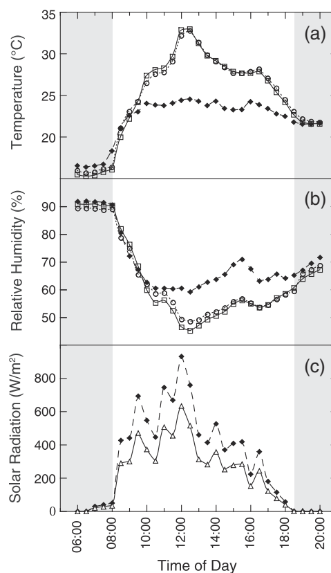
Figure 2. Temperature (a), relative humidity (b), and solar radiation (c) levels of the ambient (circles) and elevated (squares) chambers, and the open-air conditions outside the shaded greenhouse (diamonds). Shaded areas indicate nighttime, non-shaded areas indicate daytime. Uncertainty associated with the temperature and relative humidity gauge was \pm 0.36^\circ\text{C} and \pm 3.5\% , respectively. Solar radiation was measured over a spectral range of 300 to 1100 nm with an uncertainty of \pm 10\text{ W/m}^2 . Solar radiation levels inside the chambers (triangles) were calculated using the open-air measurements and transmission ratings of the shade cloth (75%) and greenhouse film (91%).
