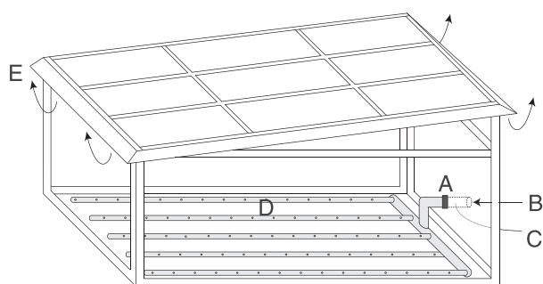
Figure 1. Controlled growth chamber design for maintenance of constant p\text{CO}_2 level, \delta^{13}\text{C}_{\text{CO}_2} value, relative humidity, and temperature. A fan located within a PVC intake pipe (A) draws ambient air (B) into the chamber. \text{CO}_2 from a gas cylinder bleeds into the intake pipe via a stainless steel capillary line (C) in order to elevate the chamber air to the desired p\text{CO}_2 level. The air is evenly distributed within the chamber via a perforated PVC manifold (D). Air is exhausted through the top of the chamber through a gap between the main structure and the roof. A 10 cm overhang of polyethylene greenhouse film provides a drip and wind guard (E). Access to the chamber is via removable side panels.
