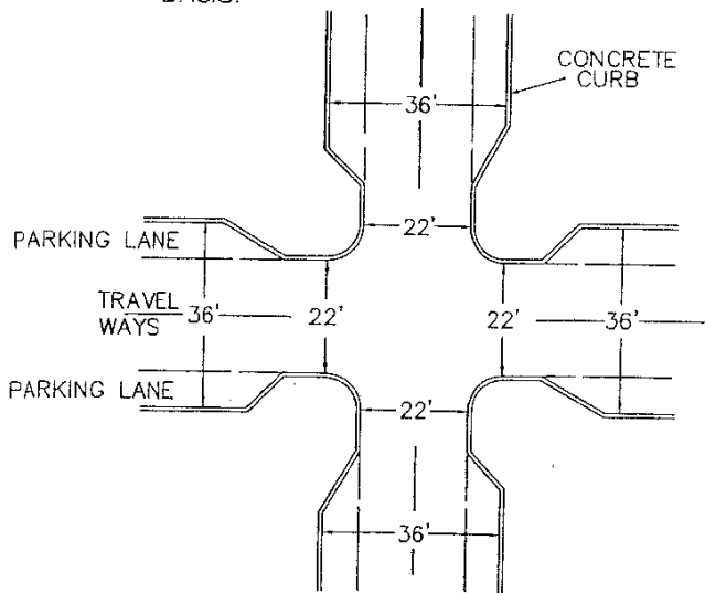
INTERSECTION DETAIL
