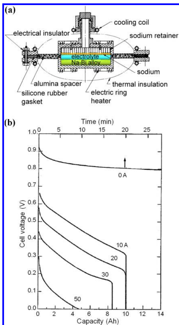
Figure 9. A Na/NaF–NaCl–Na/Bi bimetallic secondary cell developed at Argonne National Laboratory: (a) schematic of a 20 Ah nominal capacity cell with externally cooled seal and (b) plot of cell voltage versus capacity at various constant-current discharge rates of a cell at 580 °C with a 45 cm 2 electrode area and 0.4 cm interelectrode distance. Reprinted with permission from ref 37. Copyright 1967 Argonne National Laboratory.
