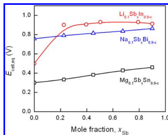
Figure 14. Plots of A|A–B–B' equilibrium cell voltages as a function of antimony mole fraction for ternary alloy systems (A–B–B'), where Li–Sb–In ternary alloys were measured for Li 0.1 In 0.9 alloys at 360–415 °C, 91,99,145,146 Na–Sb–Bi ternary alloys for Na 0.1 Bi 0.9 alloys at 577 °C, 128 and Mg–Sb–Sn ternary alloys for Mg 0.1 Sn 0.9 alloys at 800 °C. 112
