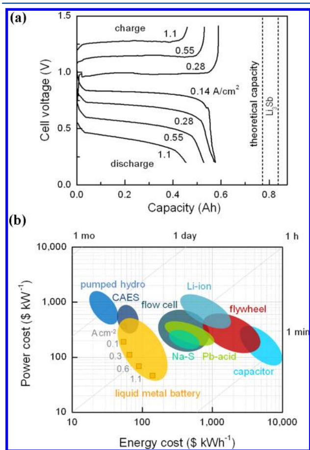
Figure 16. (a) Plot of cell voltage versus capacity upon charge and discharge at different current densities of a LiLiF–LiCl–LiIIPb–Sb cell at 450 \text{ }^\circ\text{C} with 0.77 \text{ Ah} theoretical capacity, 2.0 \text{ cm}^2 electrode area, and 1.0 \text{ cm} interelectrode distance. (b) Cost of energy versus power plot indicating various energy storage technologies (adapted from refs 8–10), where the real electrode materials costs measured for Li–Pb–Sb liquid metal battery cell are indicated by orange squares (■) and calculated from C_E^{\text{real}} = (Q_d \hat{E}_{\text{cell}})^{-1} \sum_i x_i \hat{P}_i for cost of energy and C_P^{\text{real}} = (I_d \hat{E}_{\text{cell}})^{-1} \sum_i x_i \hat{P}_i for cost of power at measured discharge current, I_d .
