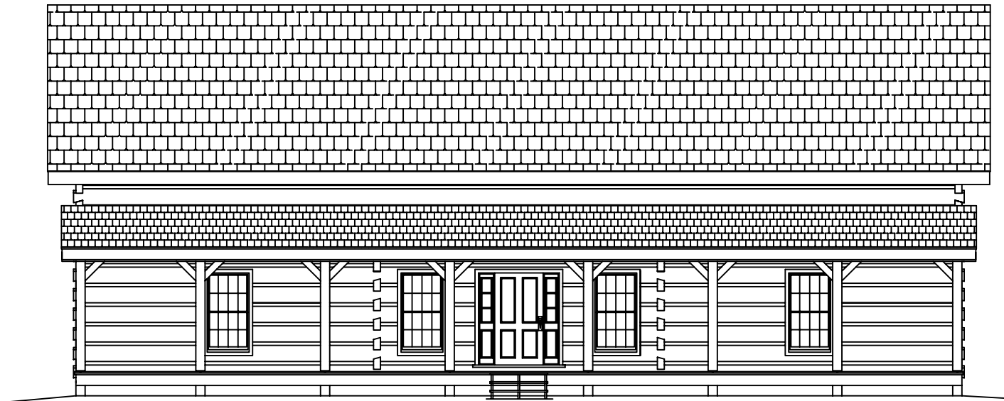
FRONT SIDE ELEVATION
