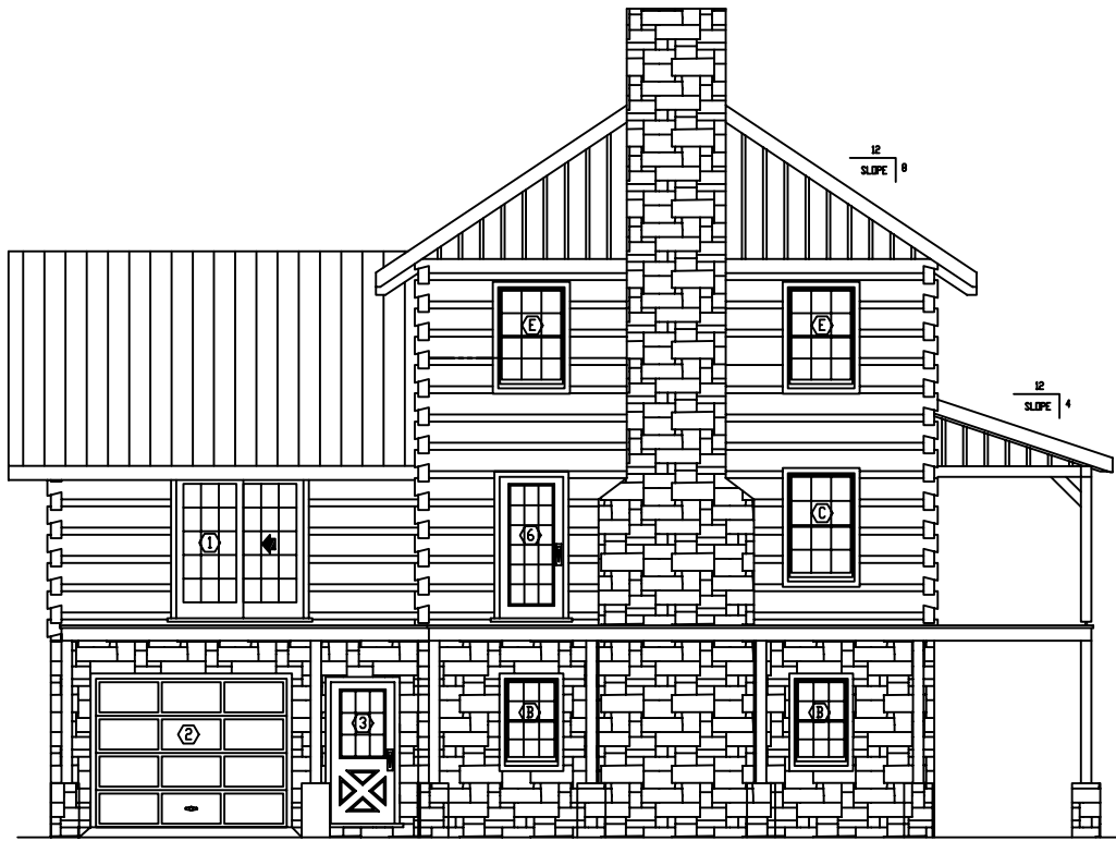
PLAN LEFT ELEVATION
