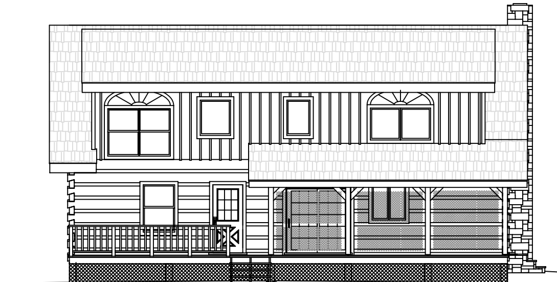
REAR ELEVATION
