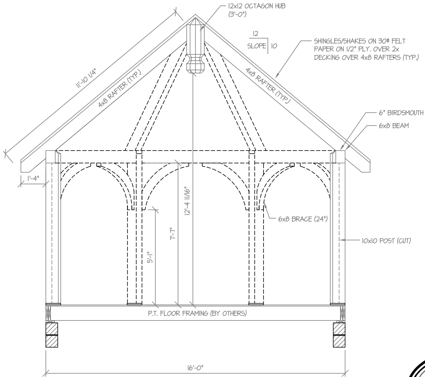
GAZEBO SECTION
