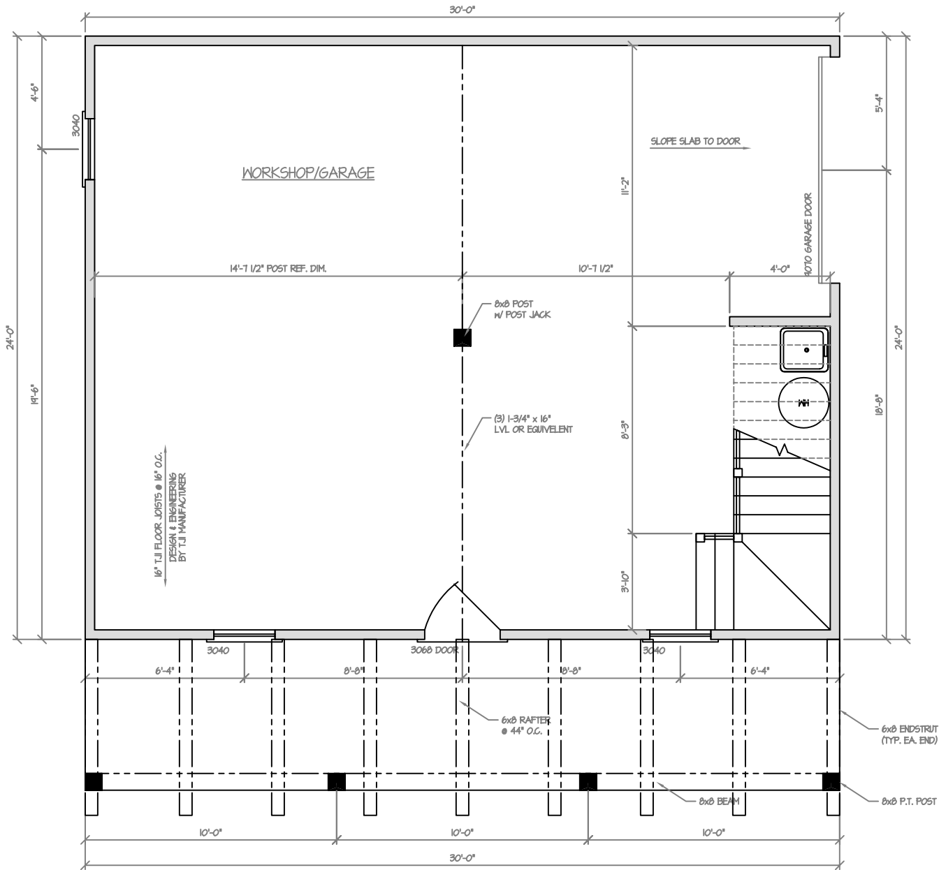
↑ PLAN FRONT FIRST FLOOR GARAGE PLAN
