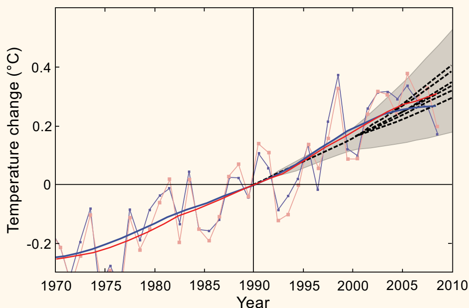
Figure 7b – Change in global average surface air temperature (smoothed over 11 years), relative to 1990. The solid blue line represents data from Hadley Center; the solid red line is GISS data. Broken lines are model projections.
