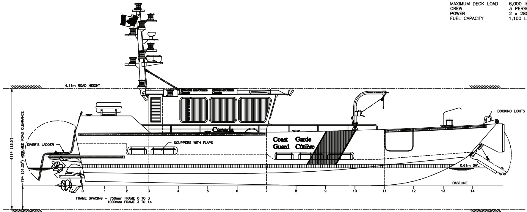
OUTBOARD PROFILE
