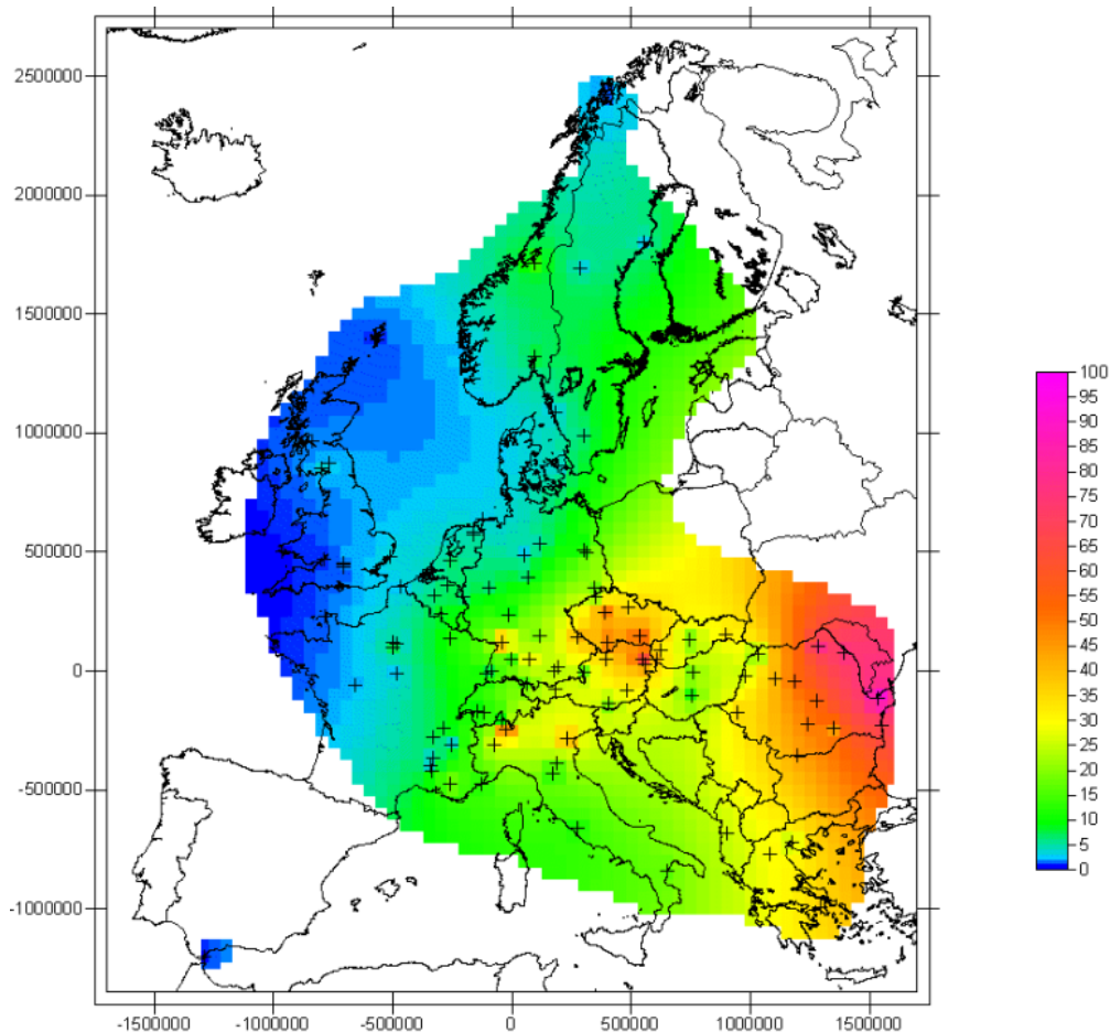
Figure 6.1 Distribution of cumulative I-131 activity concentrations in the air over Europe in May 1986 in Bq \cdot d/m^3 = becquerels x days per cubic metre of air.
