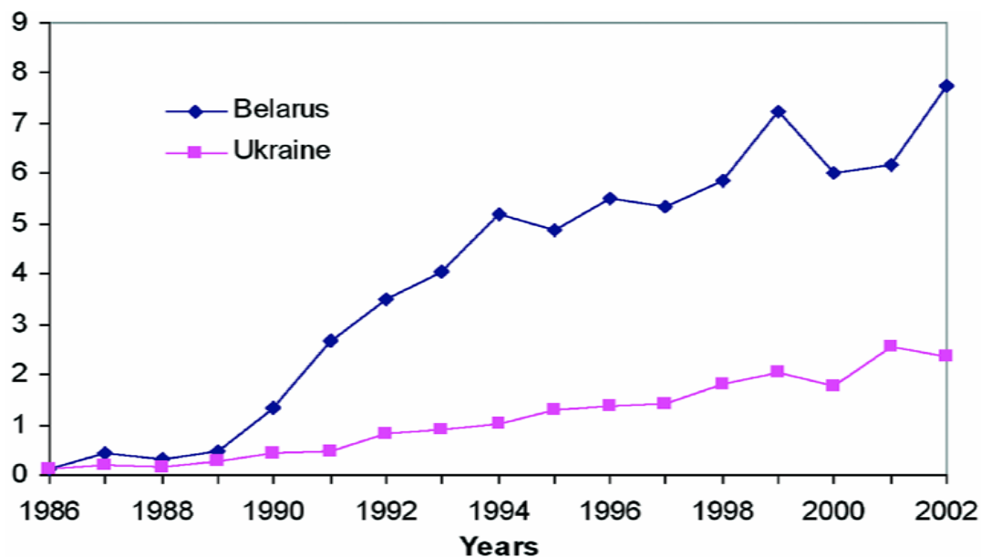
Figure 5.1. Annual thyroid cancer incidence rates per 100,000 in those who were children and adolescents under 18 years old in 1986
