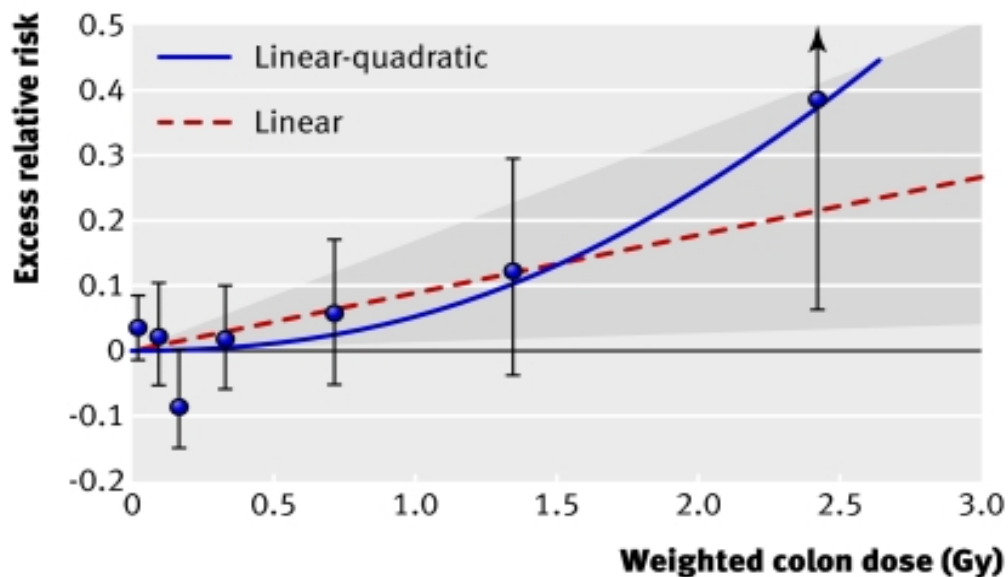
Figure 10.1 Radiation dose-response relationship (excess relative risk per Gy) for death from stroke , showing linear and linear-quadratic functions.
