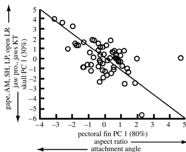
Figure 2. Plot of pectoral fin PC 1 and skull PC 1. Points are PC scores for 60 internal nodes of the labrid phylogeny and were derived from PCA on independent contrasts for pectoral fin and cranial traits. Fin PC 1 explains 80% of the total variation in fin contrasts and skull PC 1 accounts for 30% of the total variation in skull contrasts. Variables with significant PC loadings are shown on each axis, and arrows indicate their directions. These two primary axes of locomotor and cranial diversification are significantly correlated ( r = -0.53 ; p < 0.001 ).
