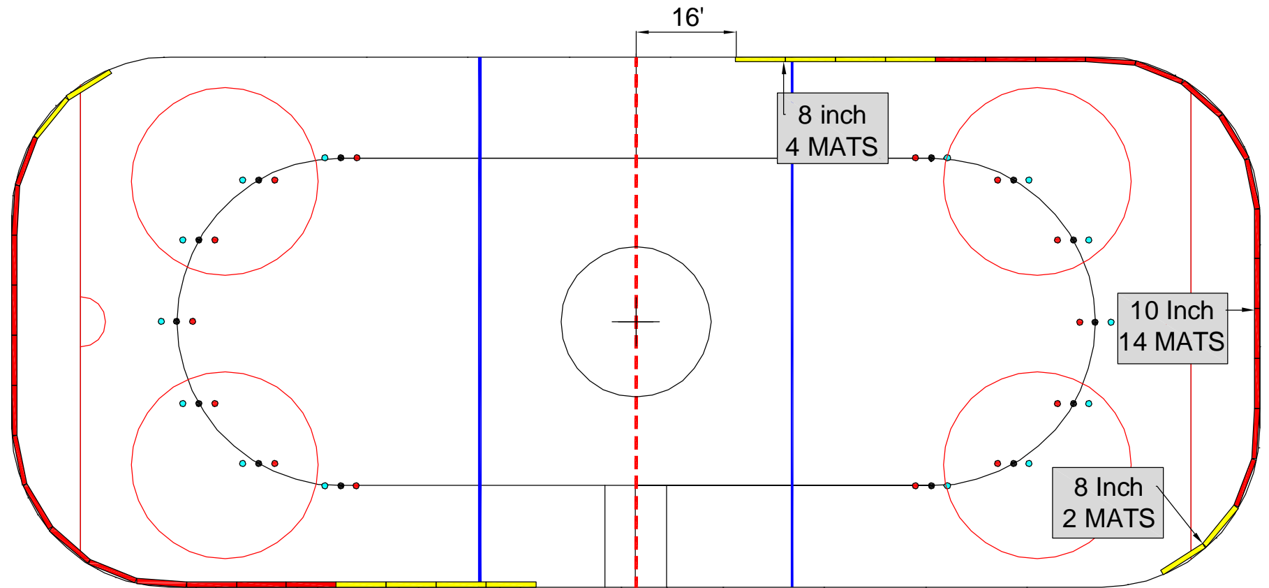
MINIMUM BOARD PAD PROTECTION FOR PRACTICES NHL SIZED ARENA 85" x 200" 111.11 METRE OVAL SHOWN MINIMUM 40 MATS REQUIRED
