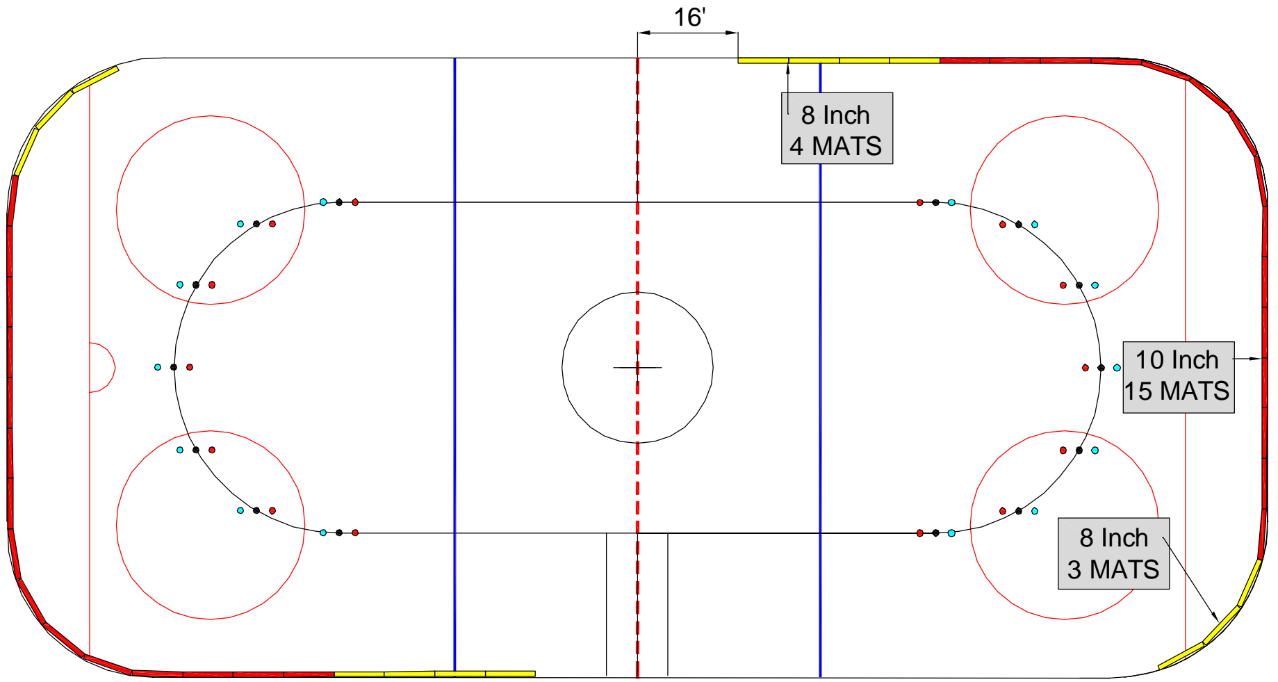
MINIMUM BOARD PAD PROTECTION FOR PRACTICES OLYMPIC SIZED ARENA 100' x 200' 111.11 METRE OVAL SHOWN MINIMUM 44 MATS REQUIRED
