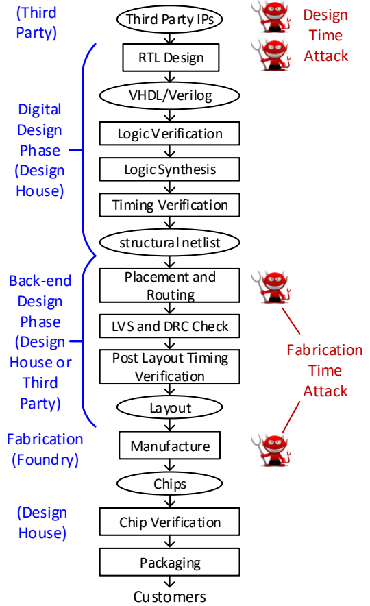
Figure 1: Typical IC design process with commonly-research threat vectors highlighted in red. Blue text and brackets highlights the party in control of the stage(s).
