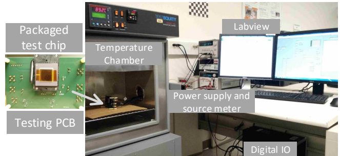
Figure 16: Testing setup for test chip measurement.
