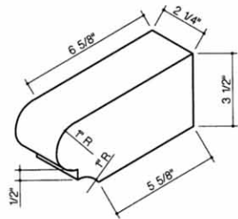
710-Rowlock Tread
