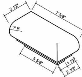
713-Rowlock Tread Corner Left
