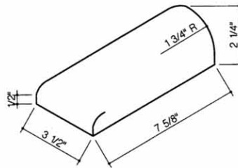
902-Coping Wall End
