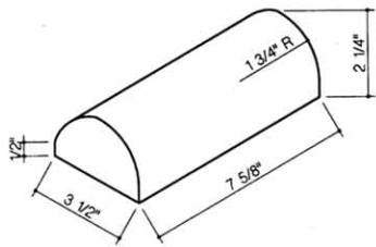
901-Coping Stretcher
