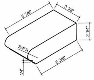
810-Header Tread
