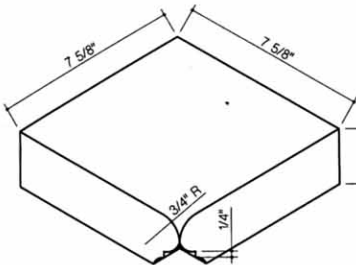
811-Header Tread Inside Corner
