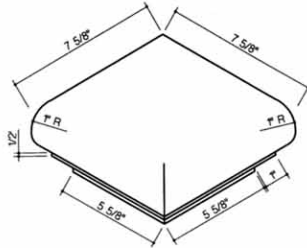
712-Rowlock Tread Outside Corner
