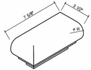
714-Rowlock Tread Corner Right
