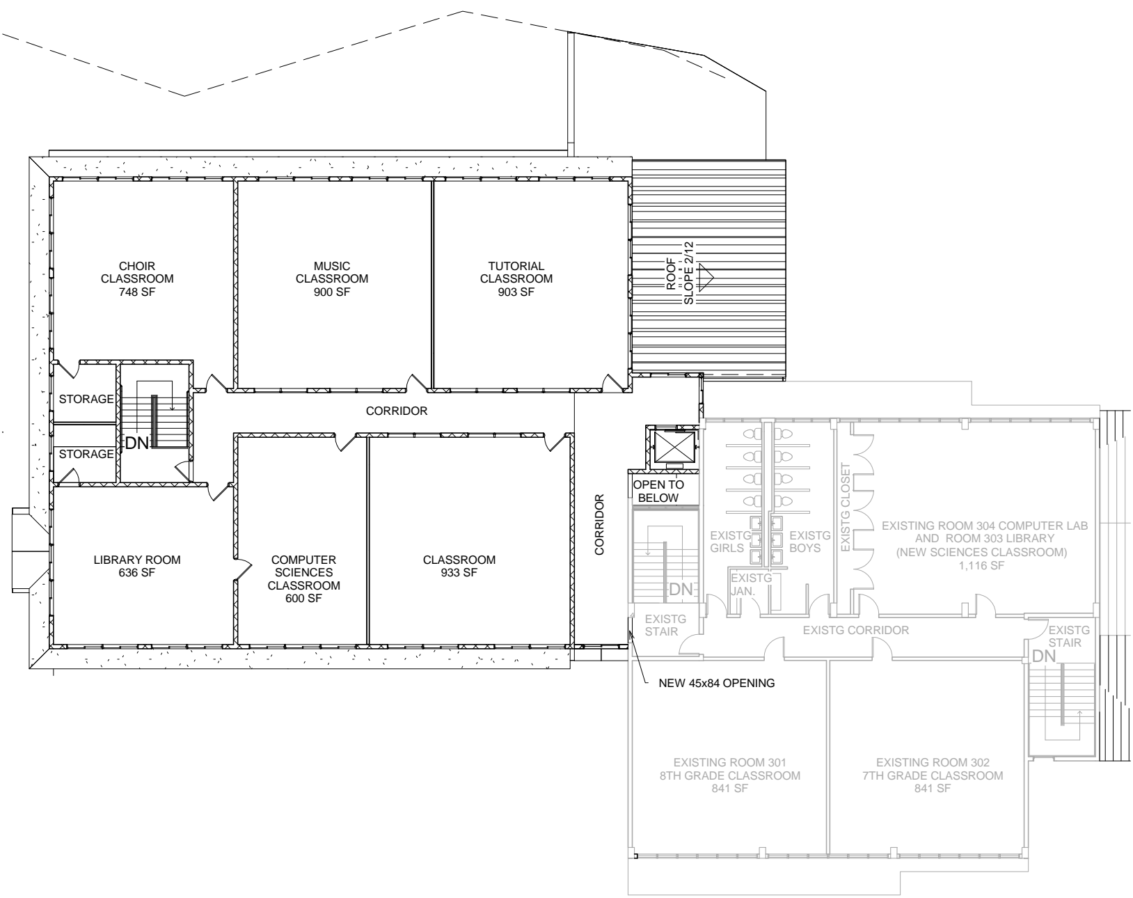
1 REMODELED 3RD FLOOR PLAN 1" = 20'-0"
