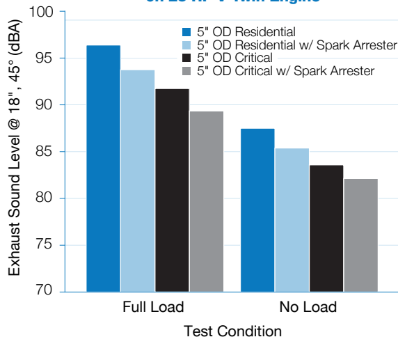
Muffler Comparison on 25 HP V-Twin Engine
