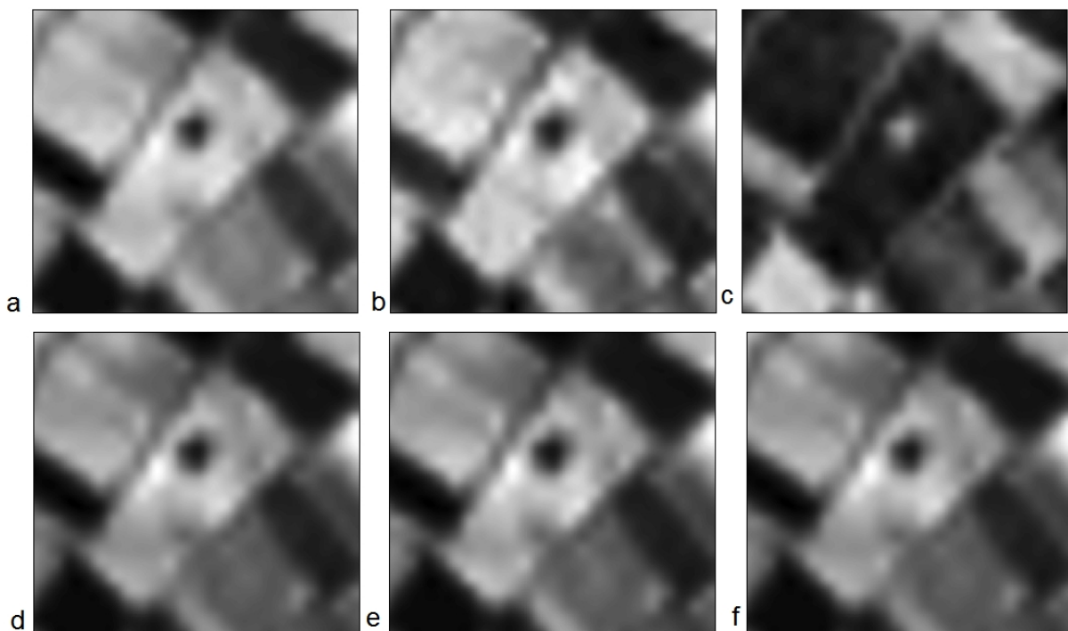
Figure 10. EO-1 HYPERION hyperspectral images used for the detection of the neolithic tell, Melia 2 , at the Thessalian plain, after the application of narrowband indices: (a) MSR 3 , (b) BRI, (c) NPCI, (d) SR 705 (e) SR and (f) SR 1 .
